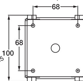
Base plate
