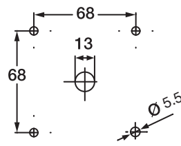
Front plate
