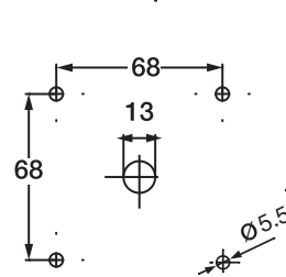
Front plate
