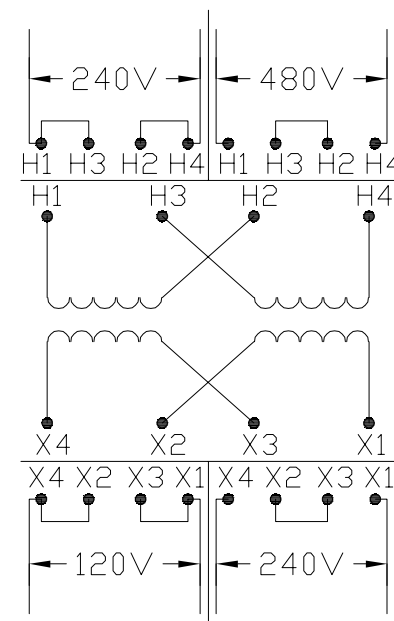
CONNECTION DIAGRAM
