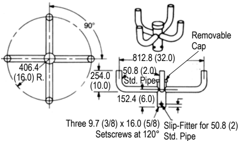
Poletop Bracket for Four Luminaires
