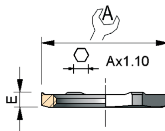
Earthing Locknut
