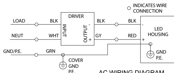
AC WIRING DIAGRAM
