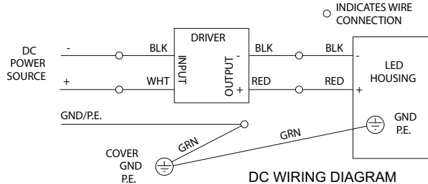
DC WIRING DIAGRAM
