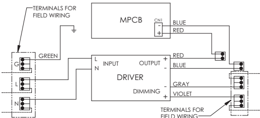
STANDARD WIRING
