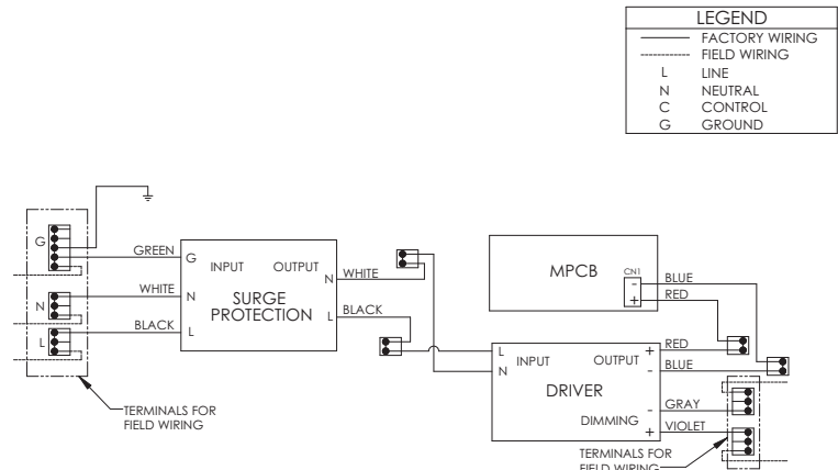
SURGE PROTECTION WIRING
