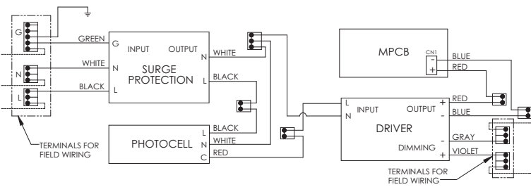
PHOTOCELL & SURGE PROTECTION WIRING
