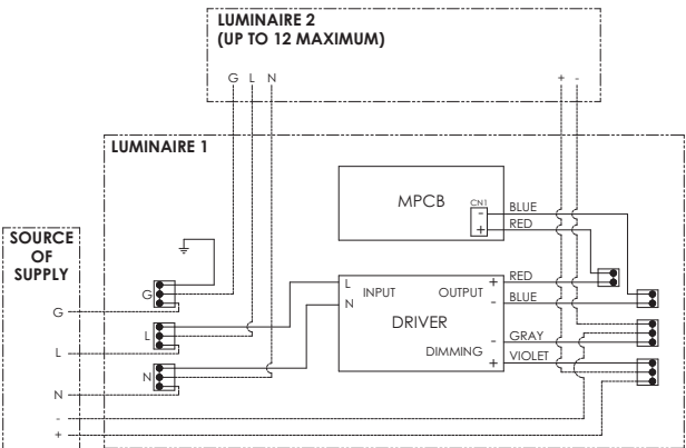
THRU-FEED WIRING
