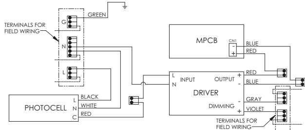
PHOTOCELL WIRING
