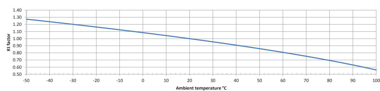
Ambient temperature
