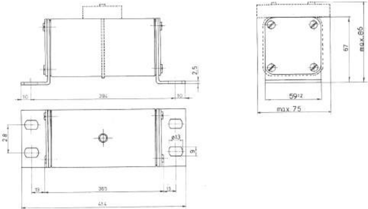
Dimensions (mm) - Size 2//2
