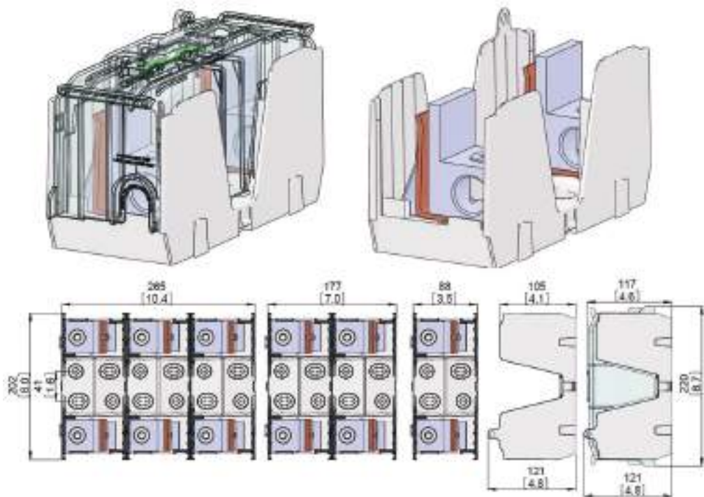
Dimensions mm (in) - 400 A
