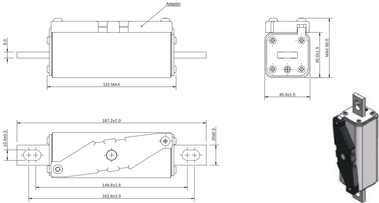
Dimensions (mm) - Size 01, bolted
