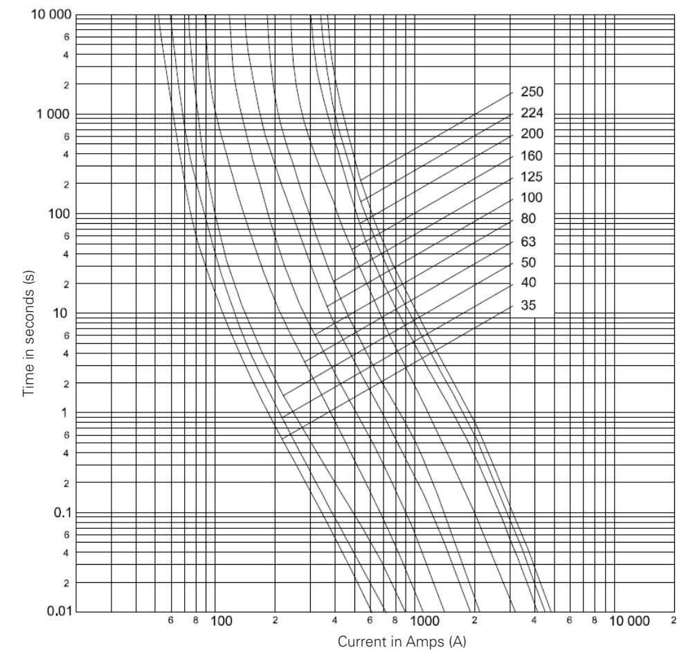
Time-current curves - NH Size 02
