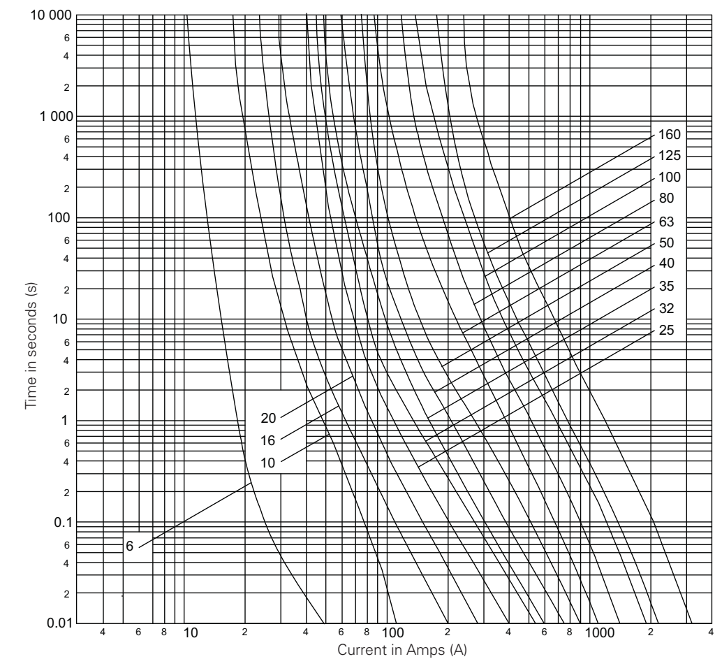
Technical data - NH size 01
