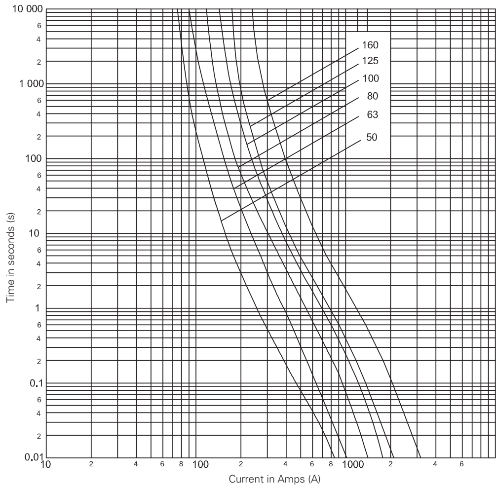
Time-current curves - NH Size 00
