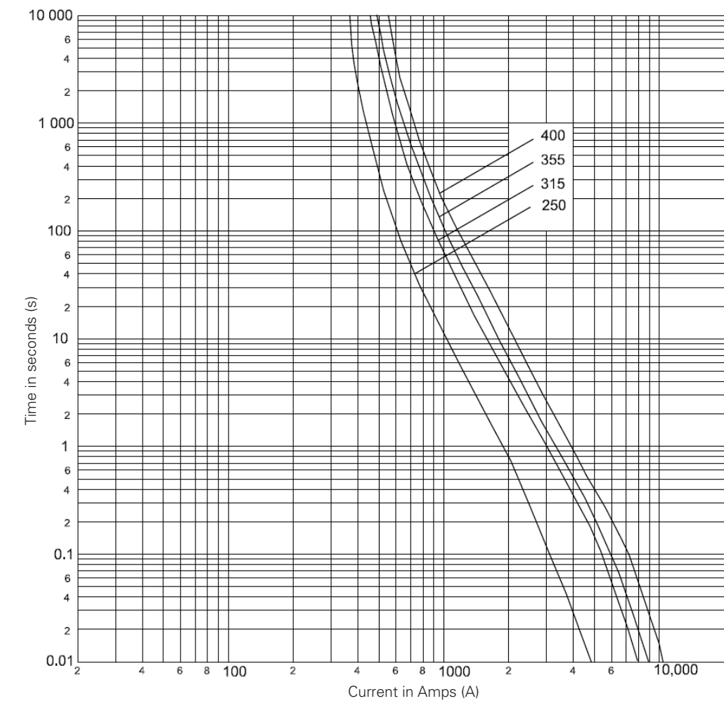
Time-current curves - NH Size 03
