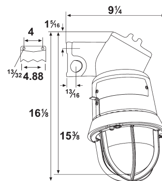
Bulkhead mount
