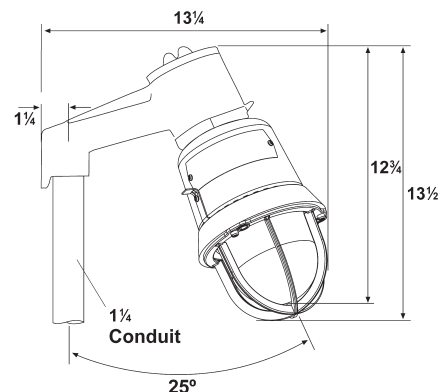
Stanchion mount
