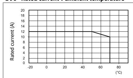
L 96 - Rated current v ambient temperature
