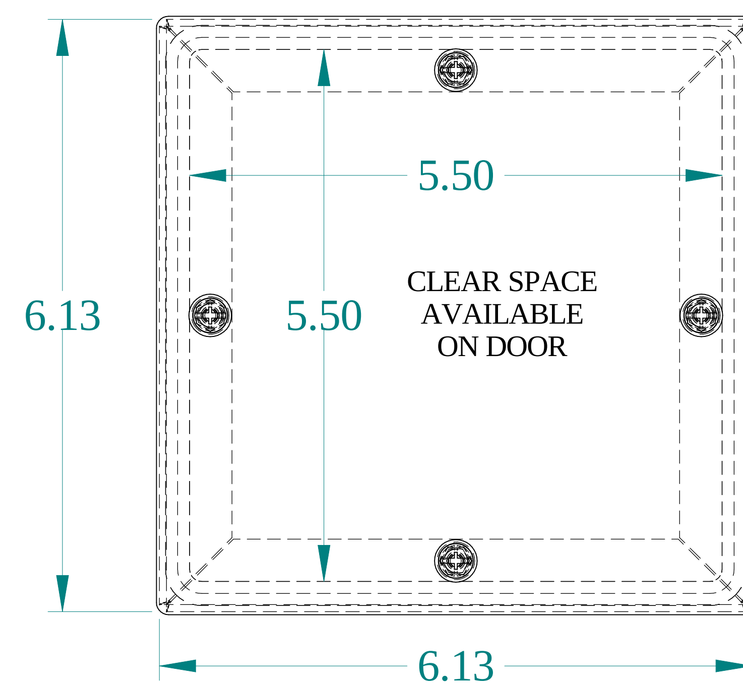
FRONT VIEW
