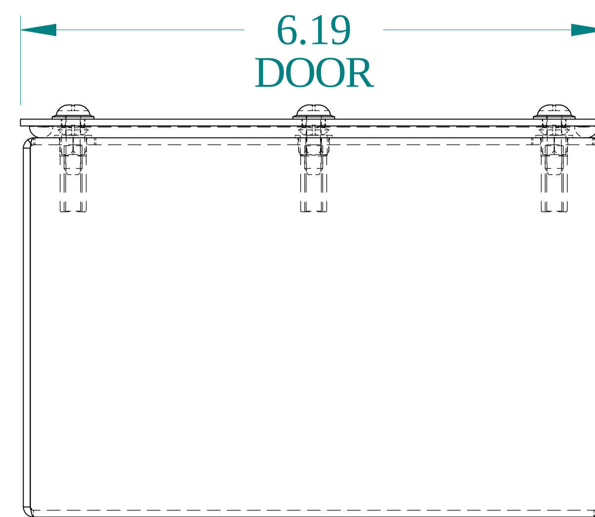
BOTTOM VIEW
