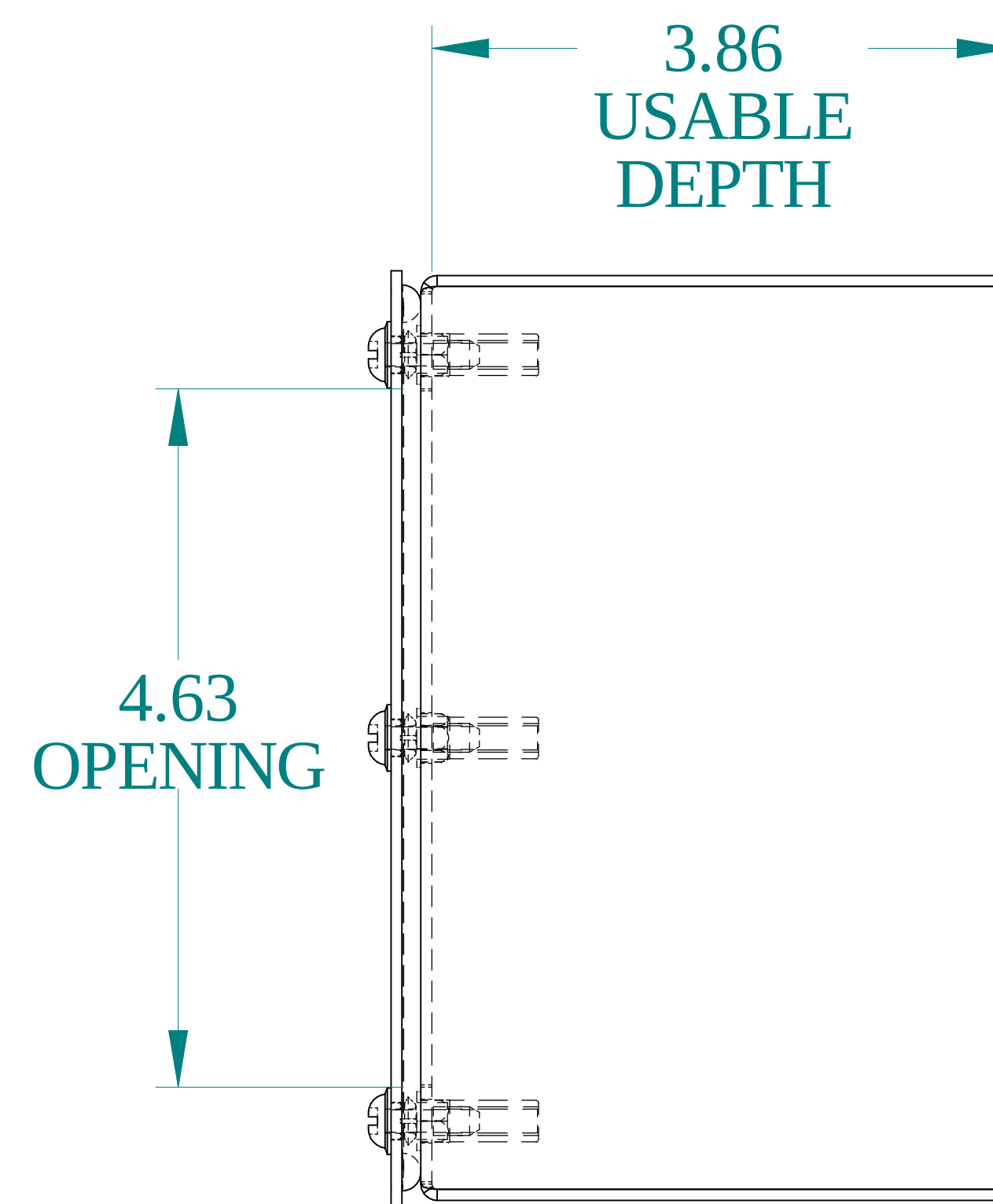
SIDE VIEW
