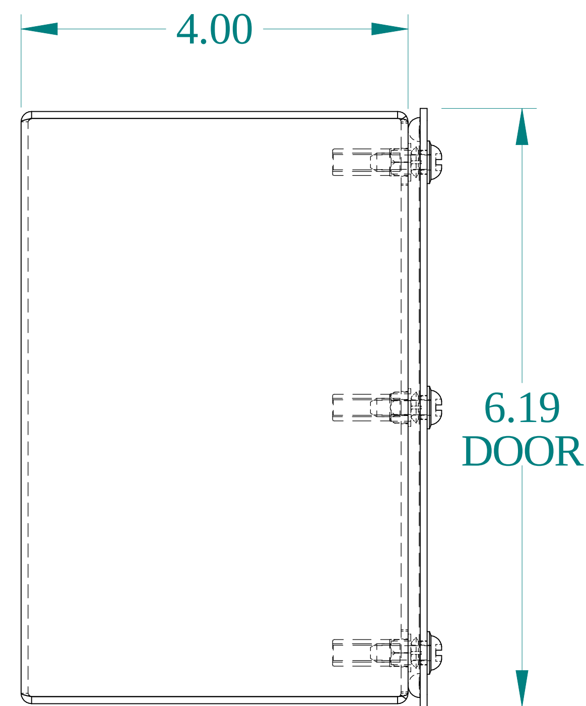
SIDE VIEW
