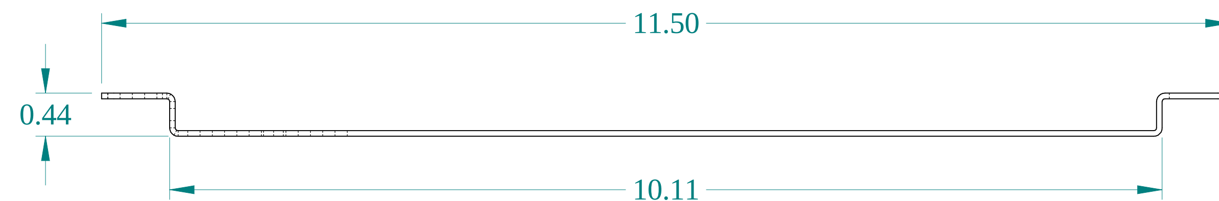
TOP VIEW
