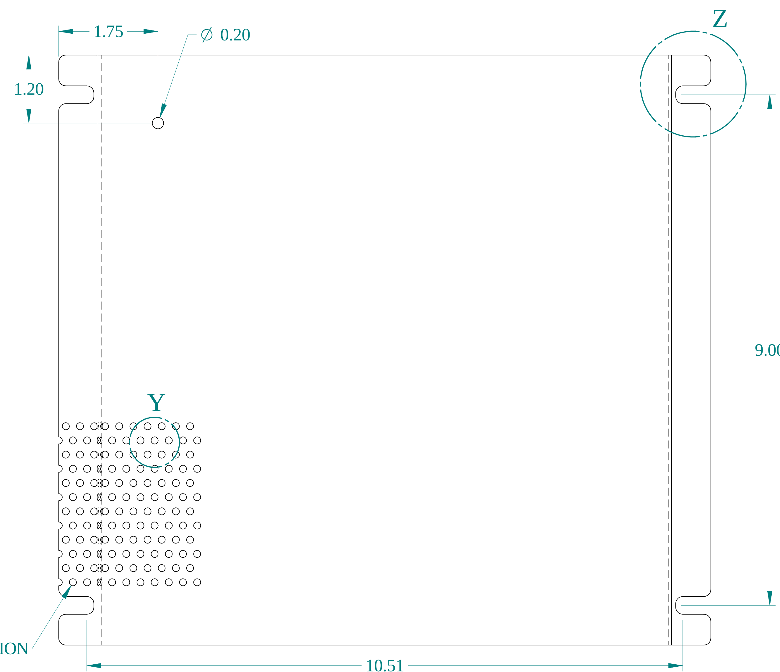
FRONT VIEW
