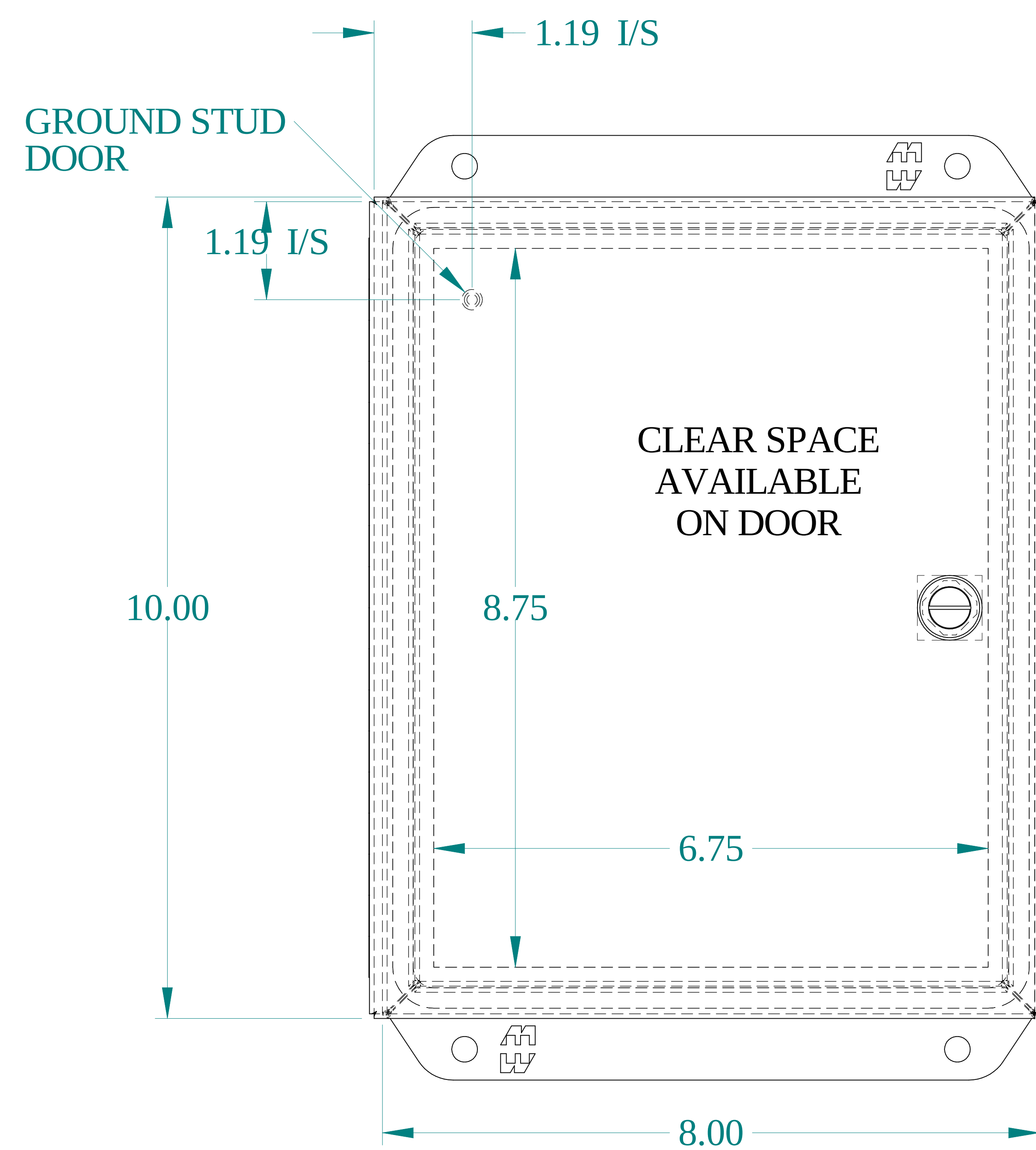
FRONT VIEW
