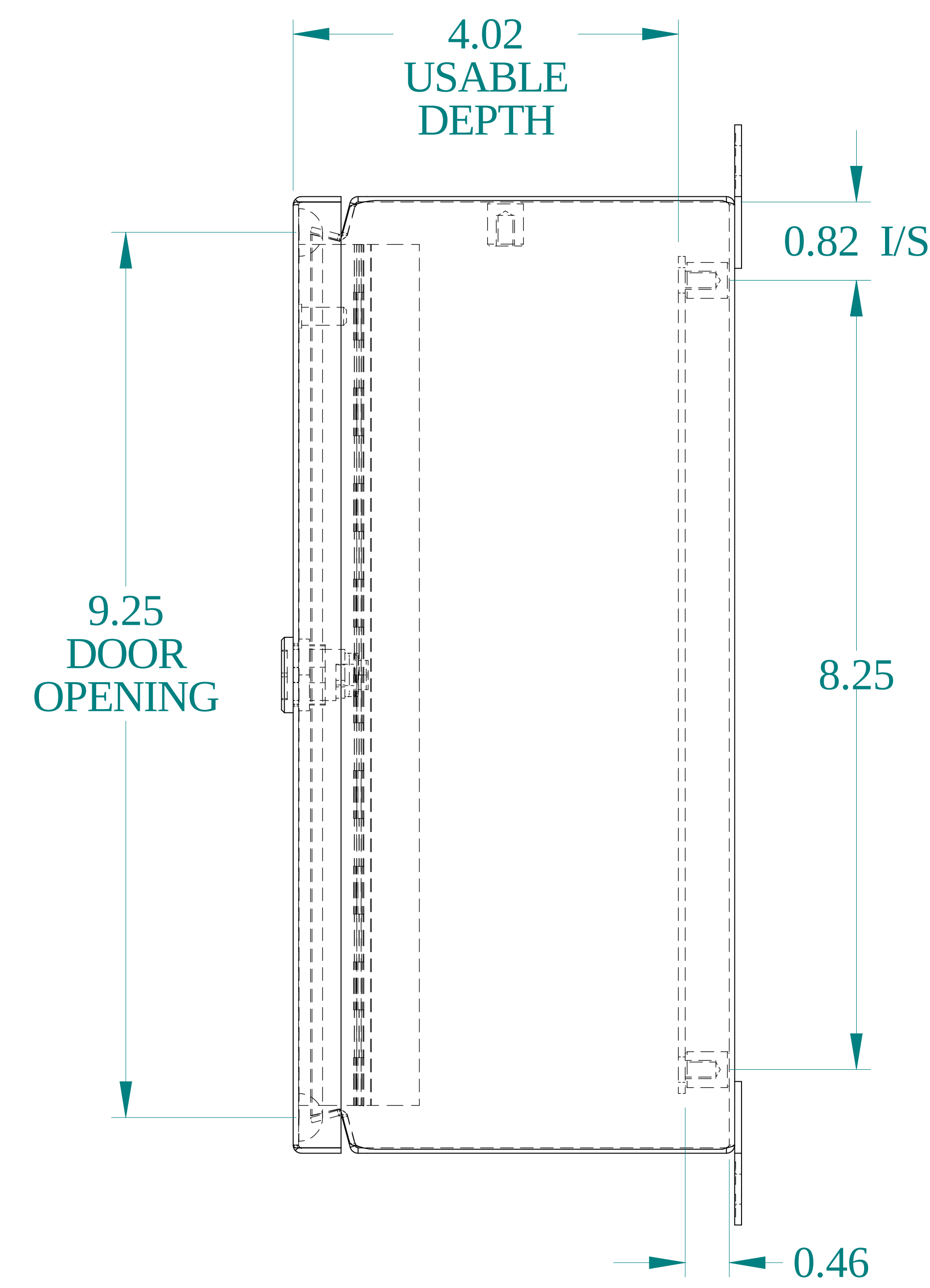
SIDE VIEW
