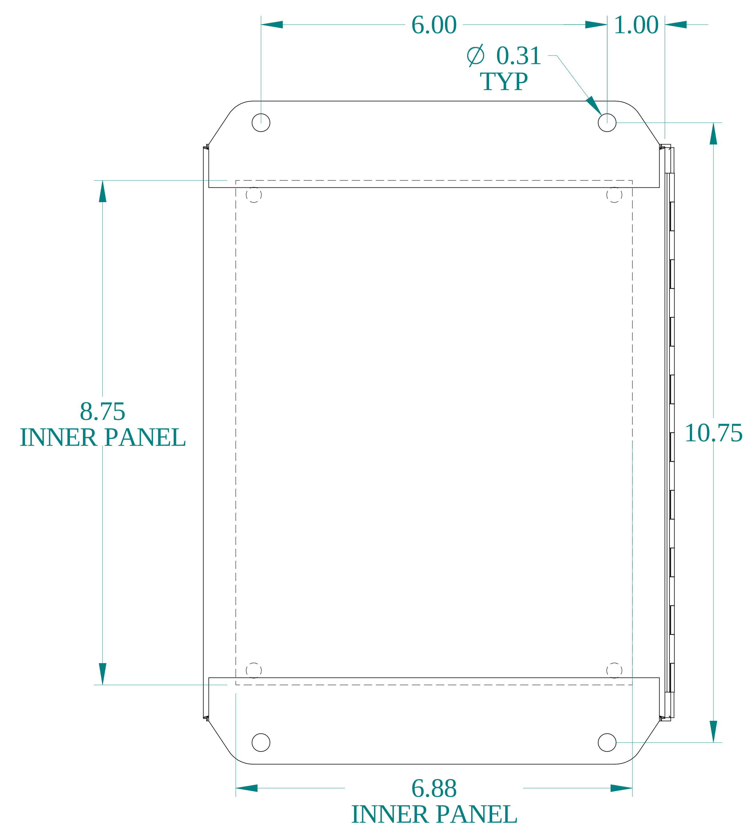
BACK VIEW
