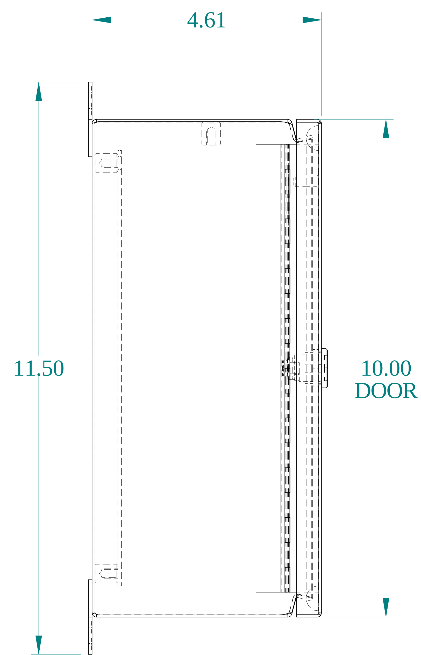
SIDE VIEW
