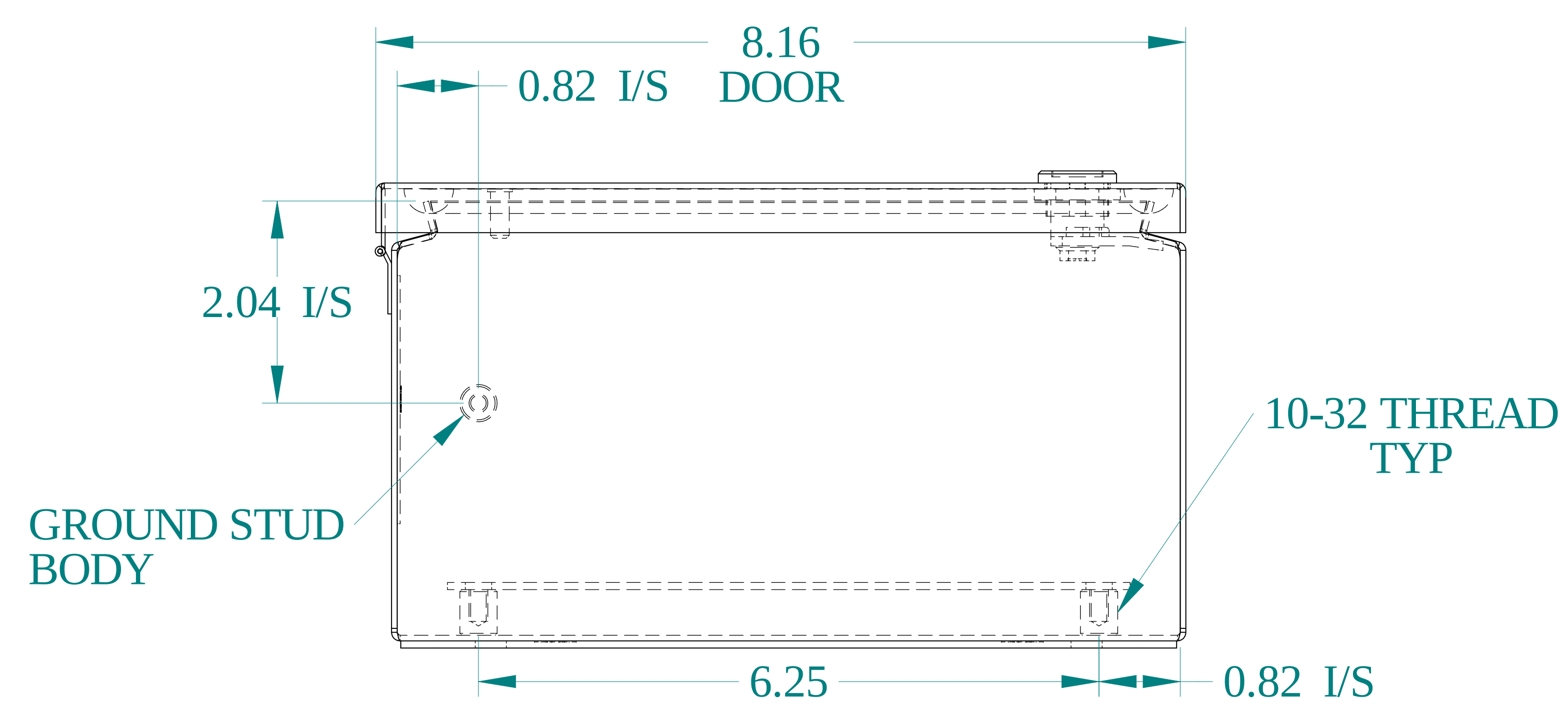
BOTTOM VIEW
