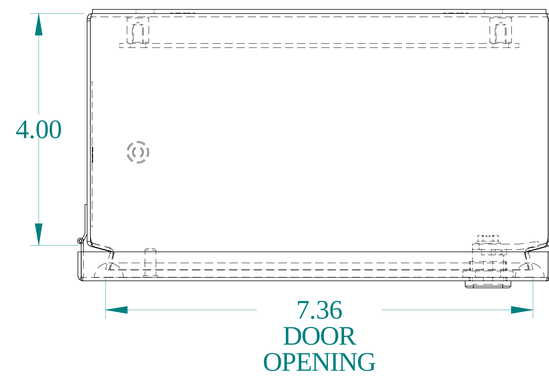
TOP VIEW
