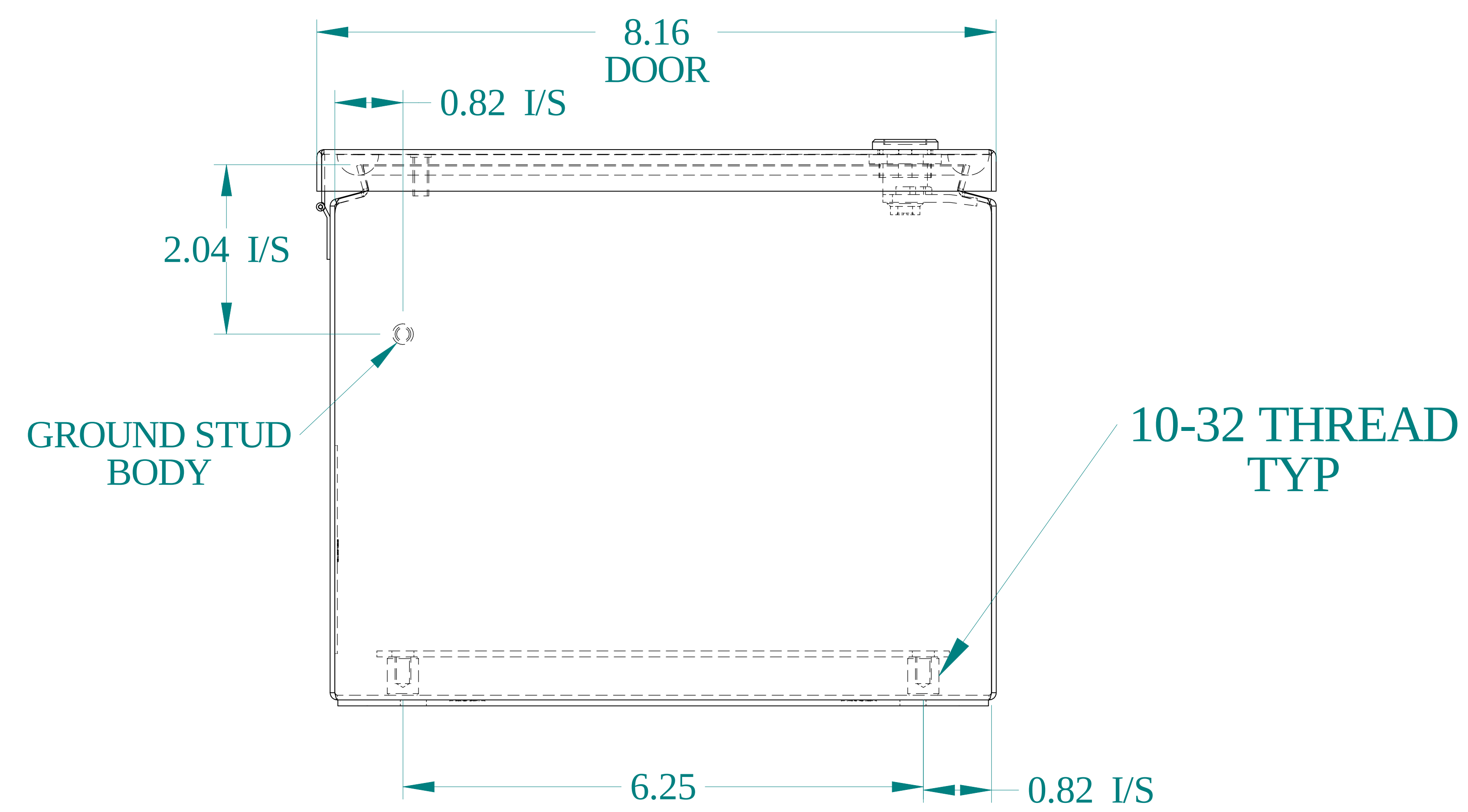
BOTTOM VIEW
