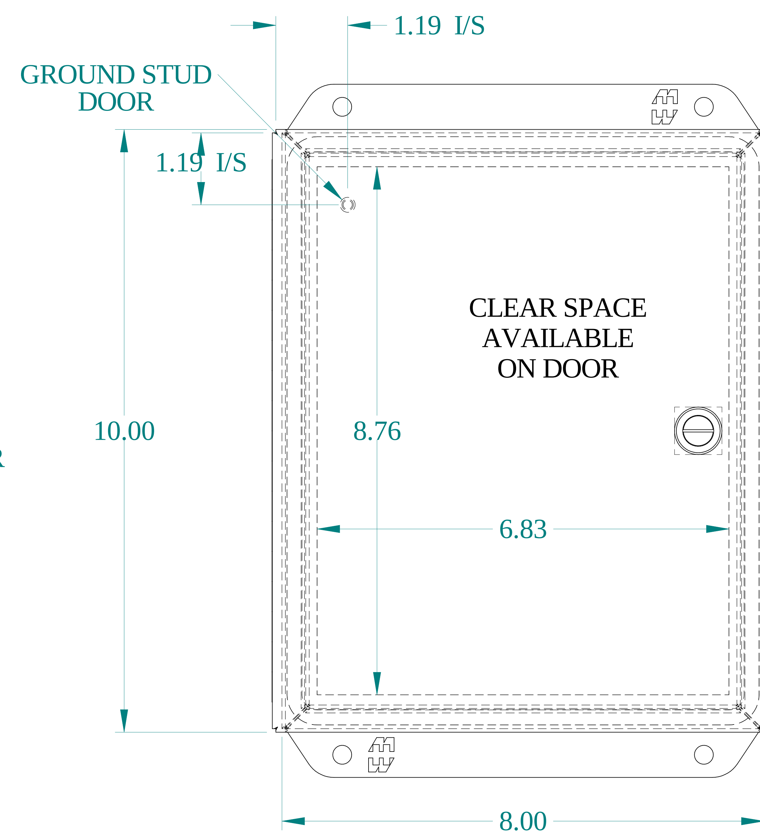
FRONT VIEW
