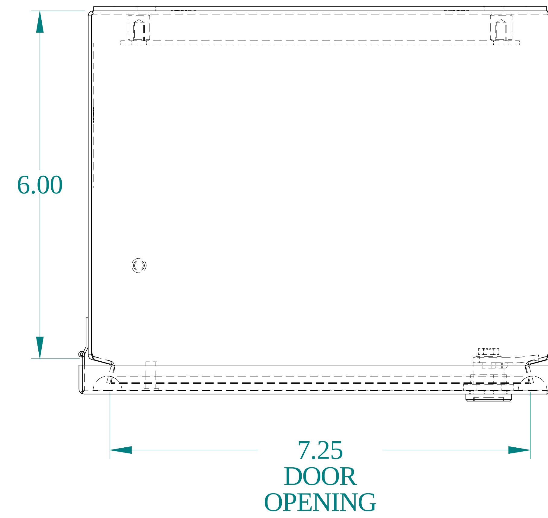
TOP VIEW
