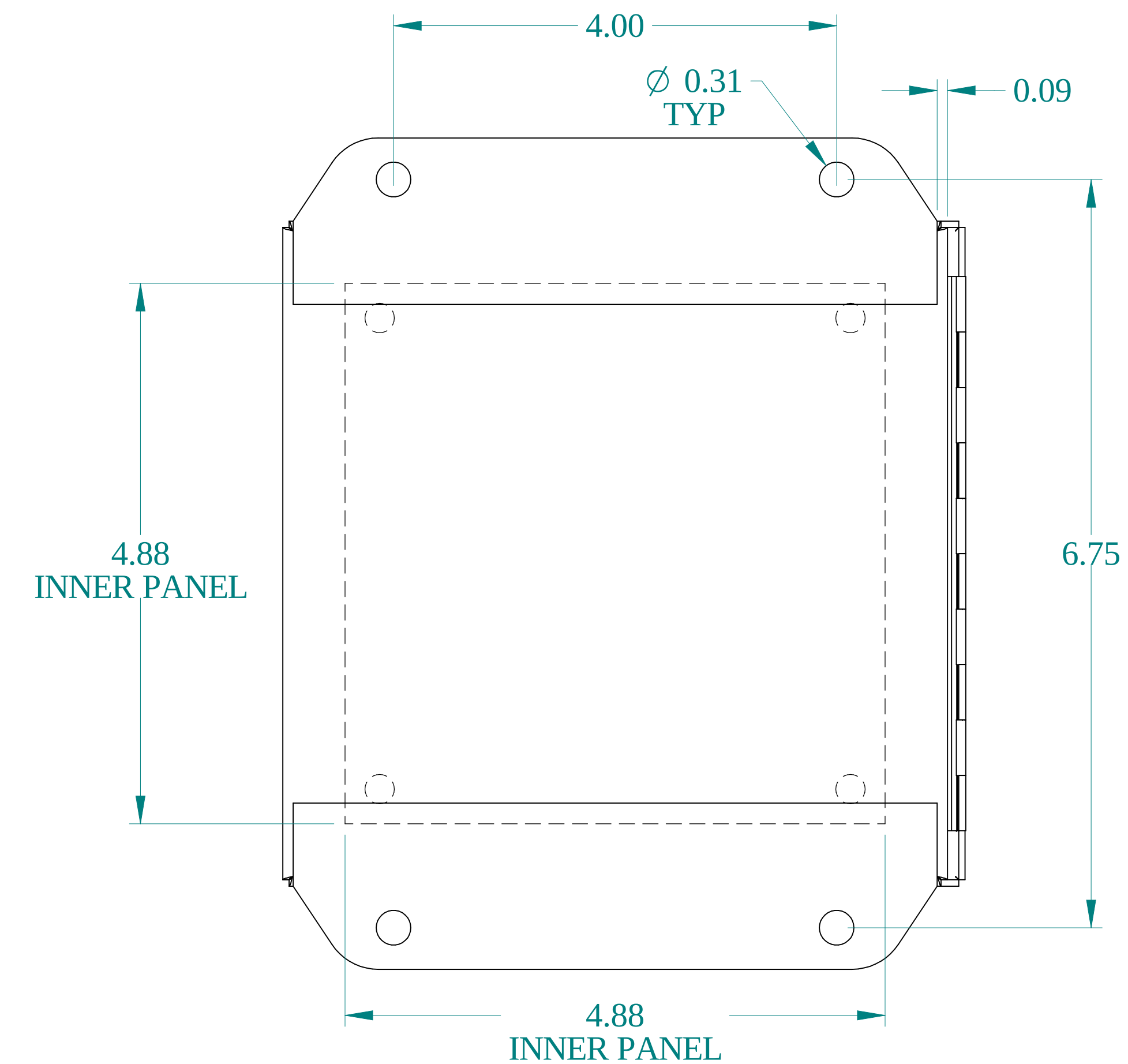
BACK VIEW
