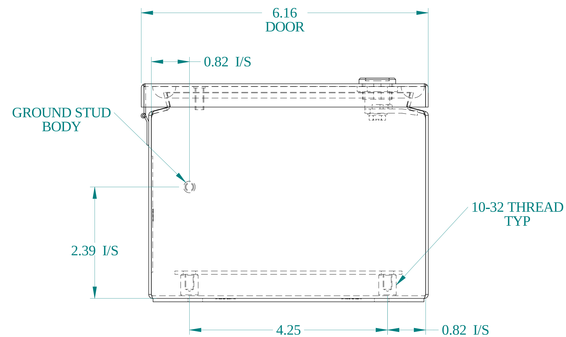
BOTTOM VIEW
