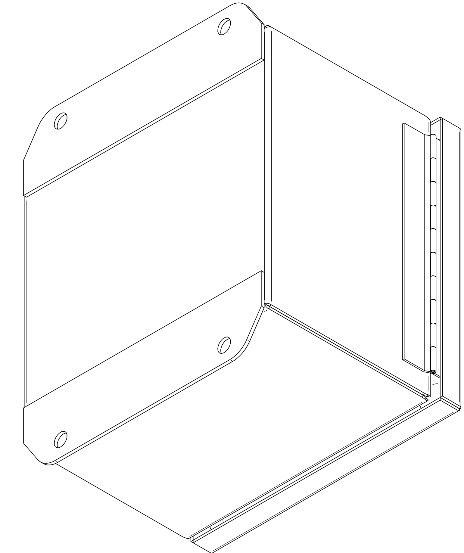
ISOMETRIC VIEWS
