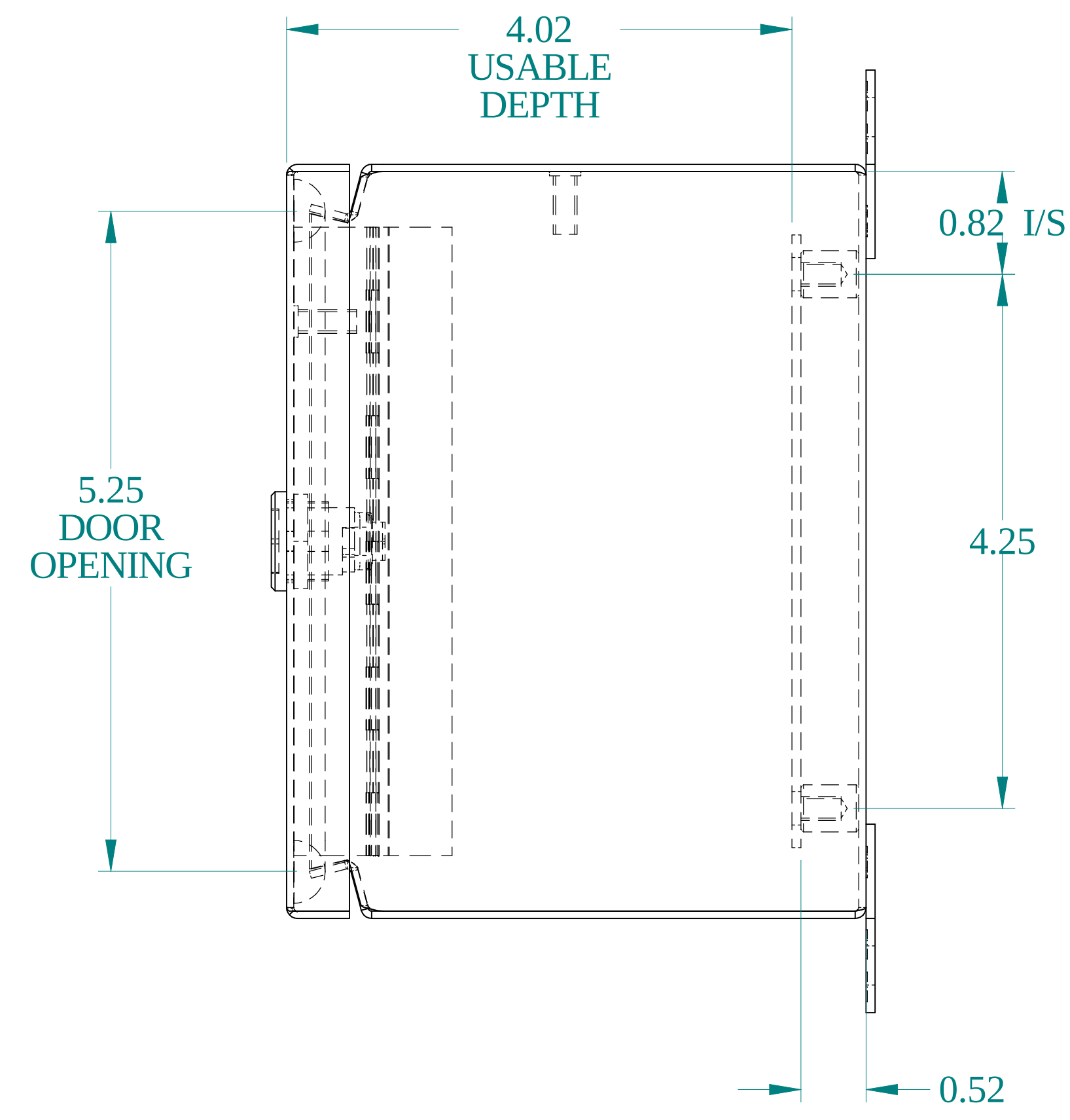
SIDE VIEW
