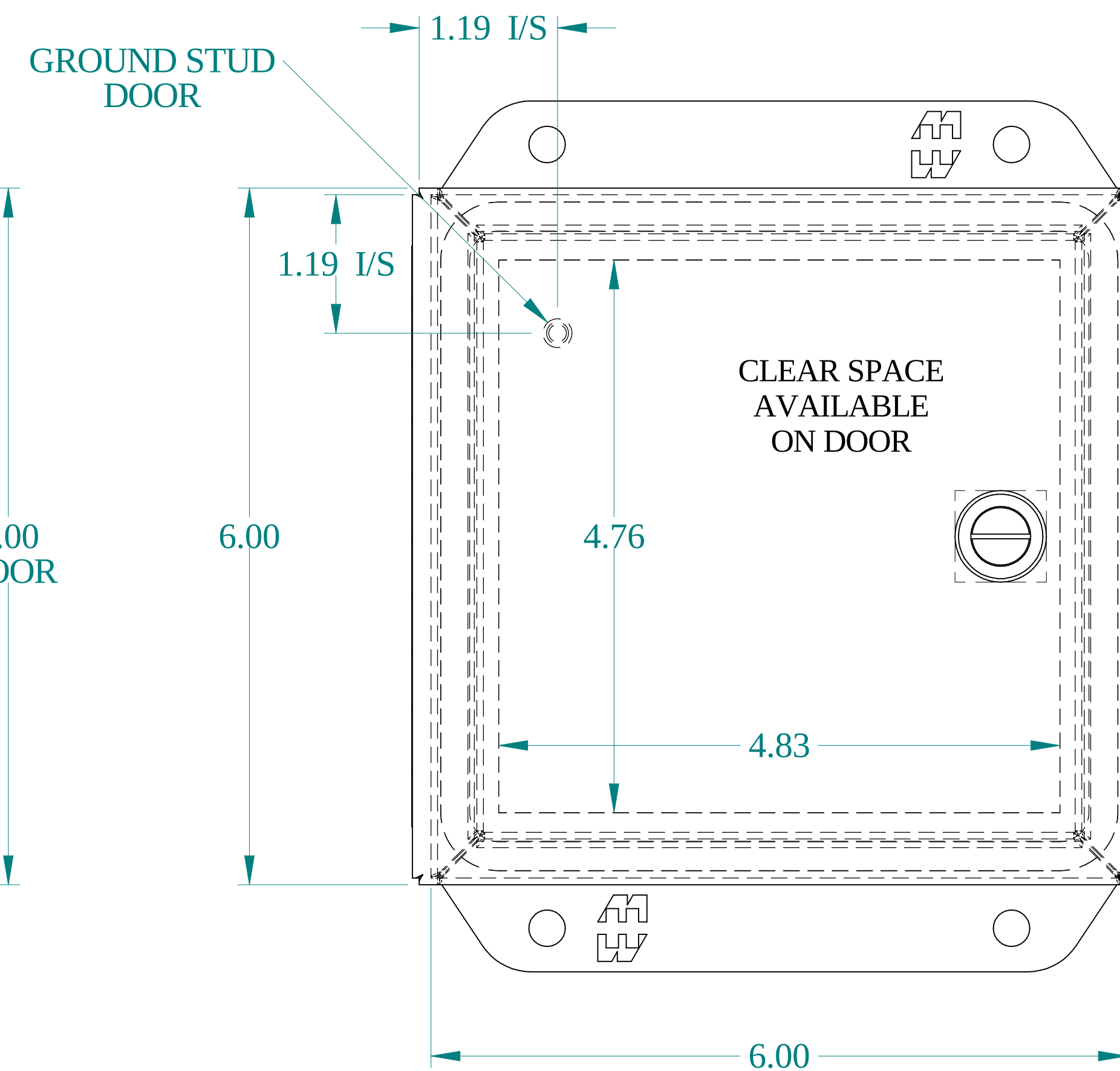
FRONT VIEW
