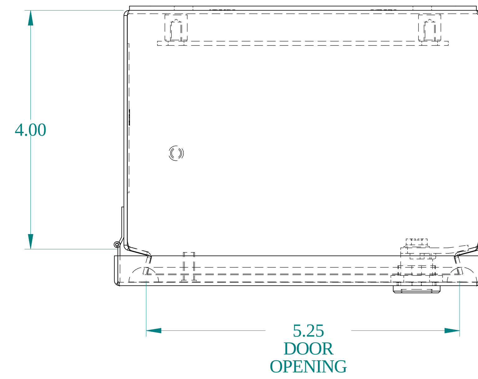
TOP VIEW
