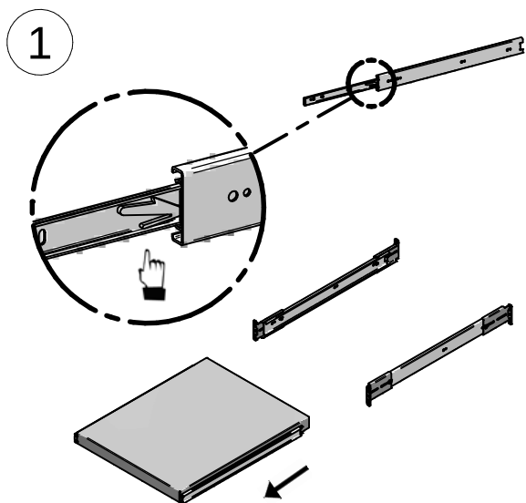
ITEM 1 PULL OUT SHELF QTY 1
