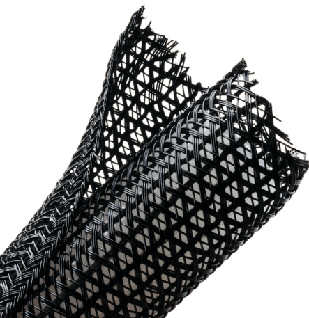
Braided Sleeving, Split Wrap, 1.25" Dia, PET, Black, 75 ft/bulk reel
