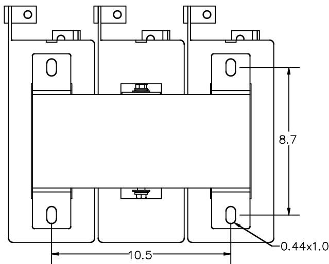
BOTTOM VIEW
