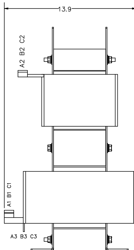
SIDE VIEW
