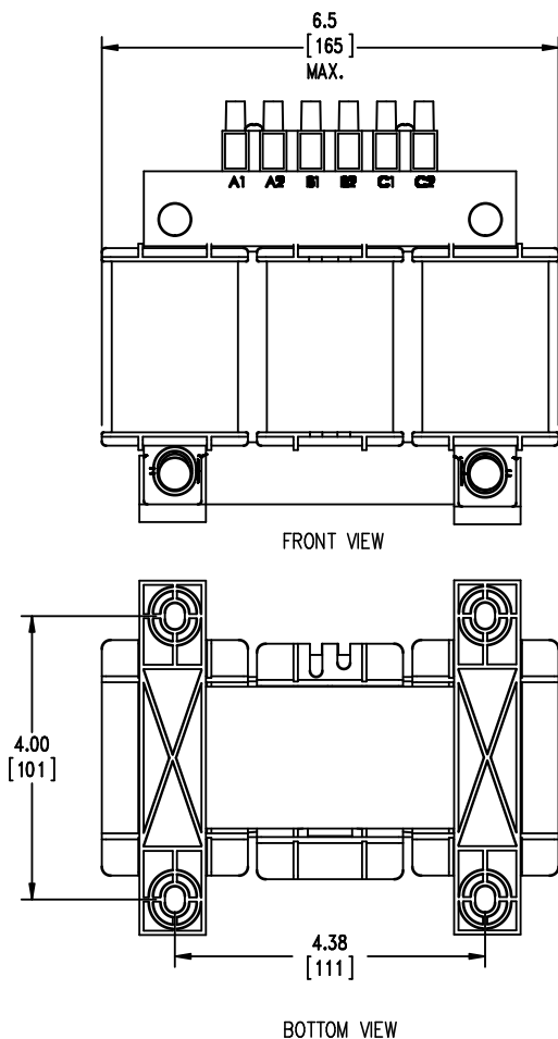
BOTTOM VIEW
