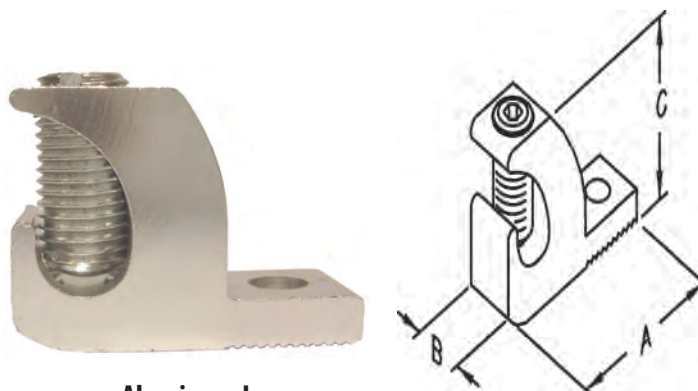
Aluminum Lugs
