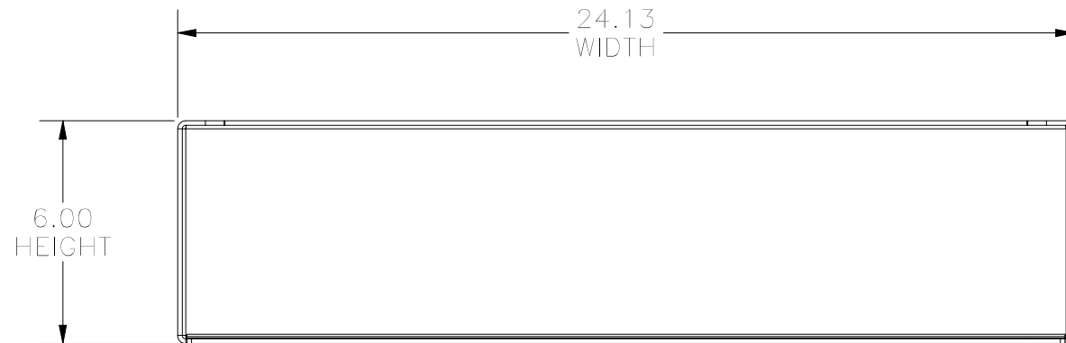
TOP VIEW
