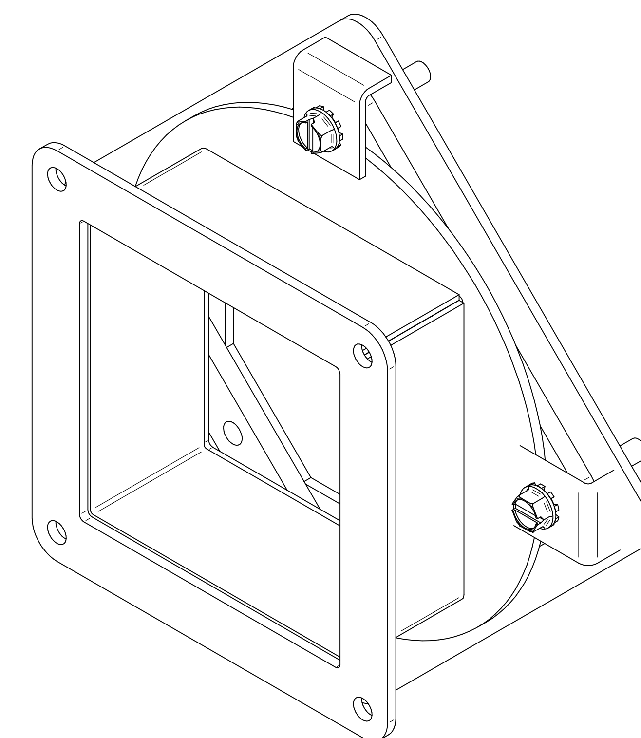
ISOMETRIC VIEW
