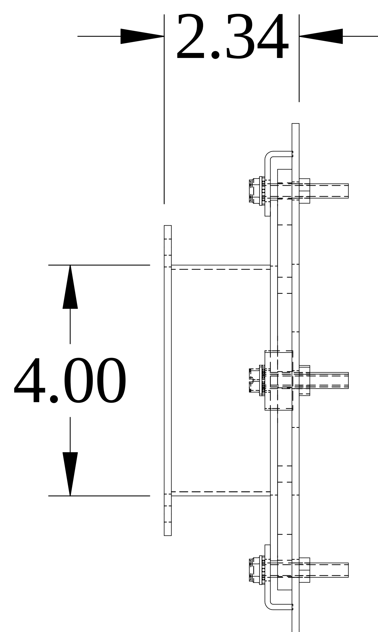
SIDE VIEW
