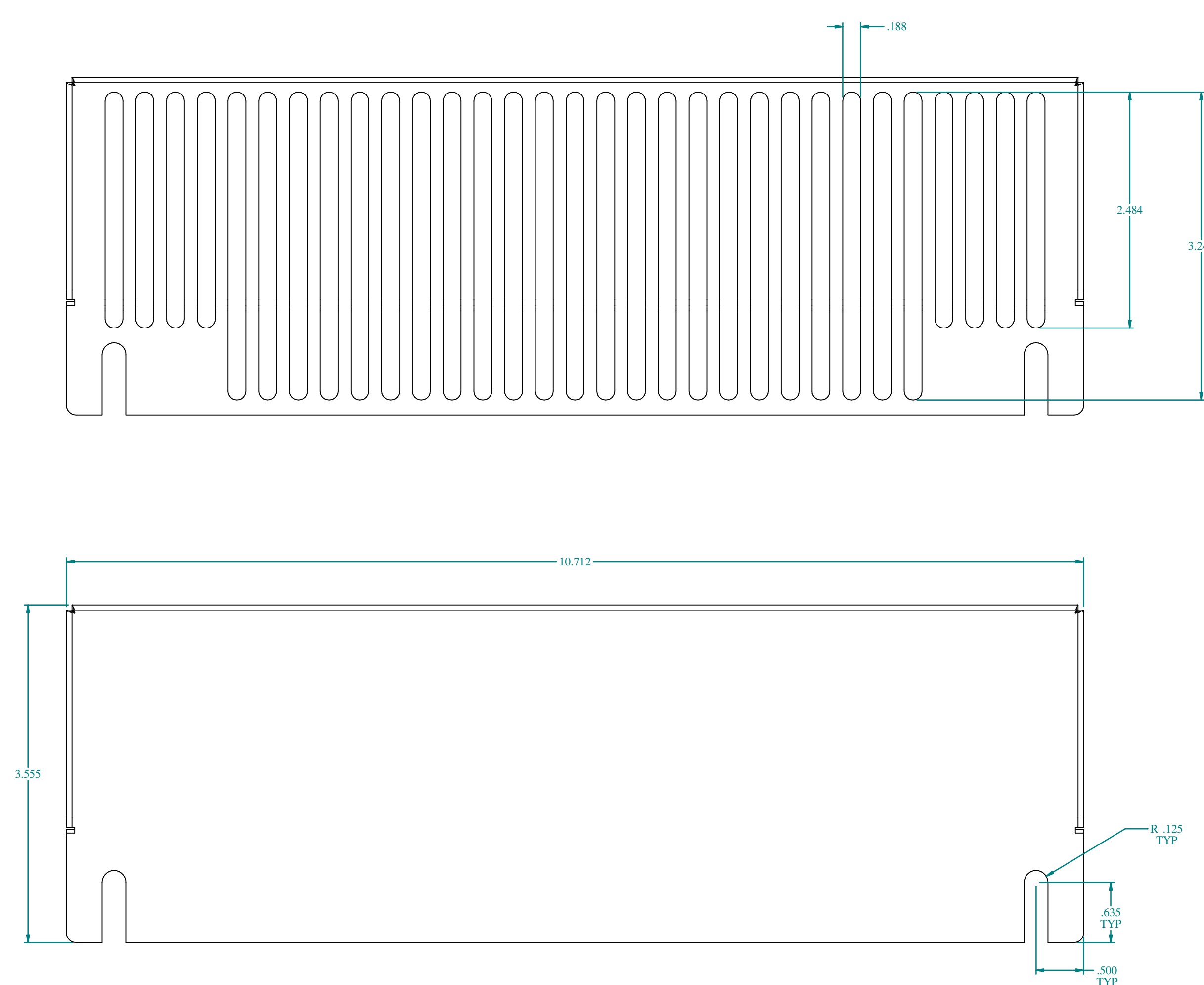
TOP VIEW
