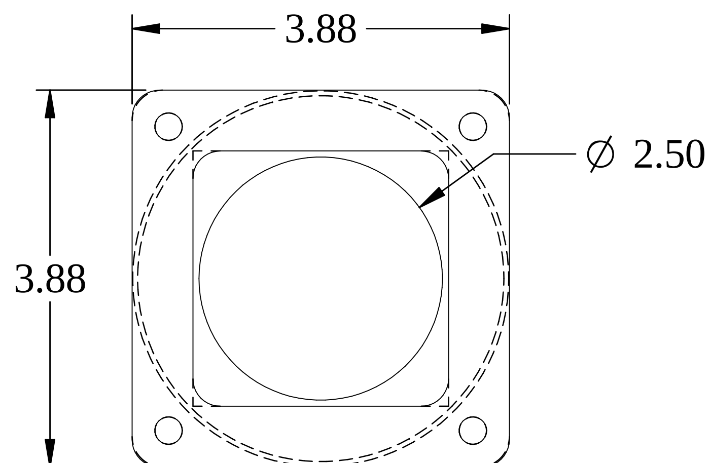
END VIEW
