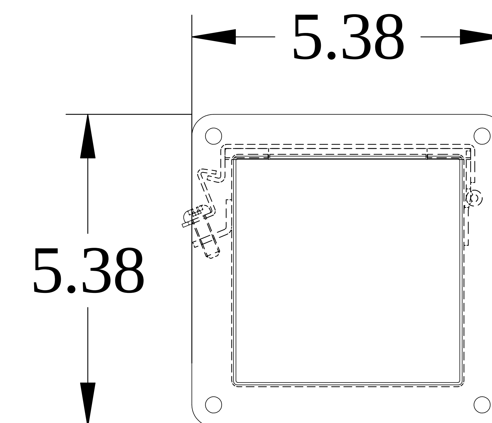
END VIEW
