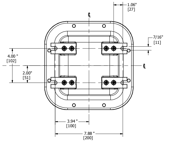
MOUNTING FEET
