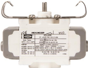
Panel mount N.O. contact block
