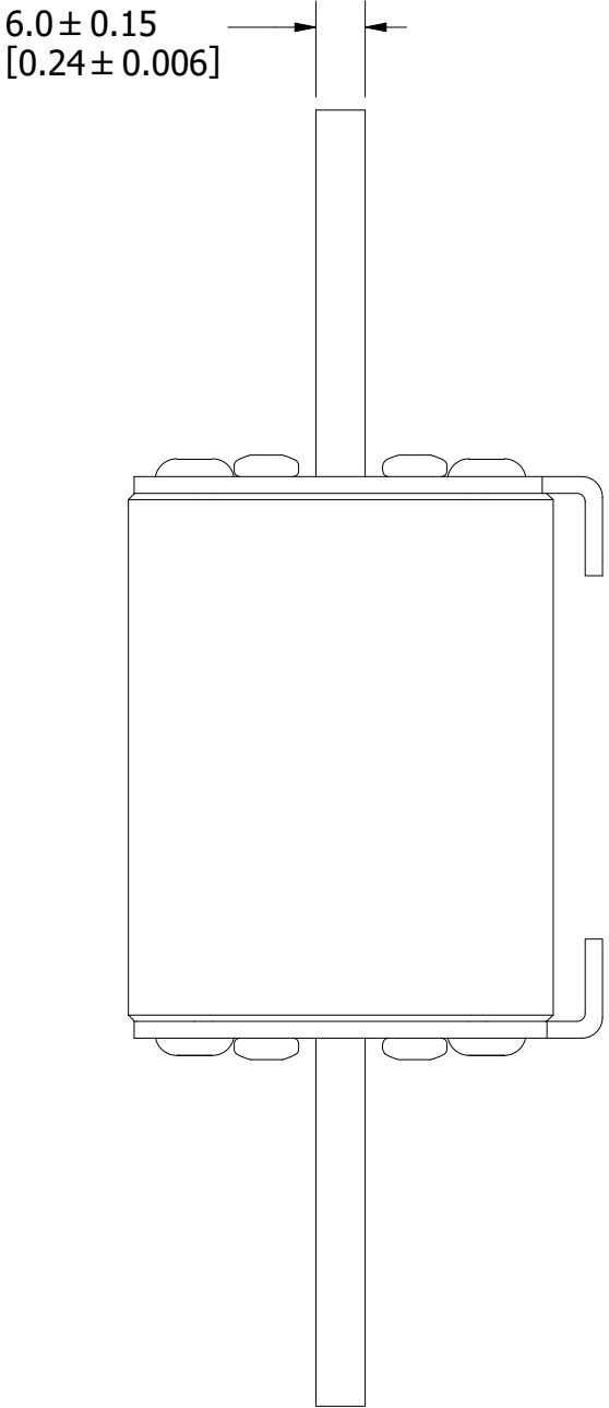
FUSE
