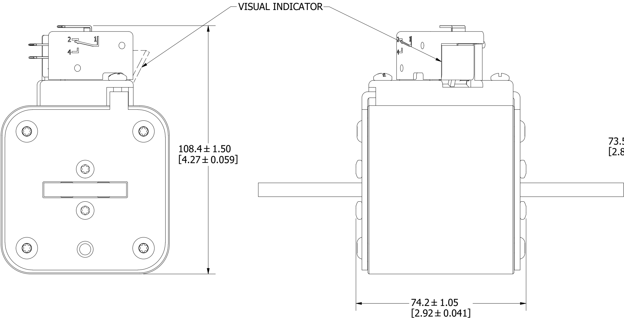
FUSE WITH MICROSWITCH
