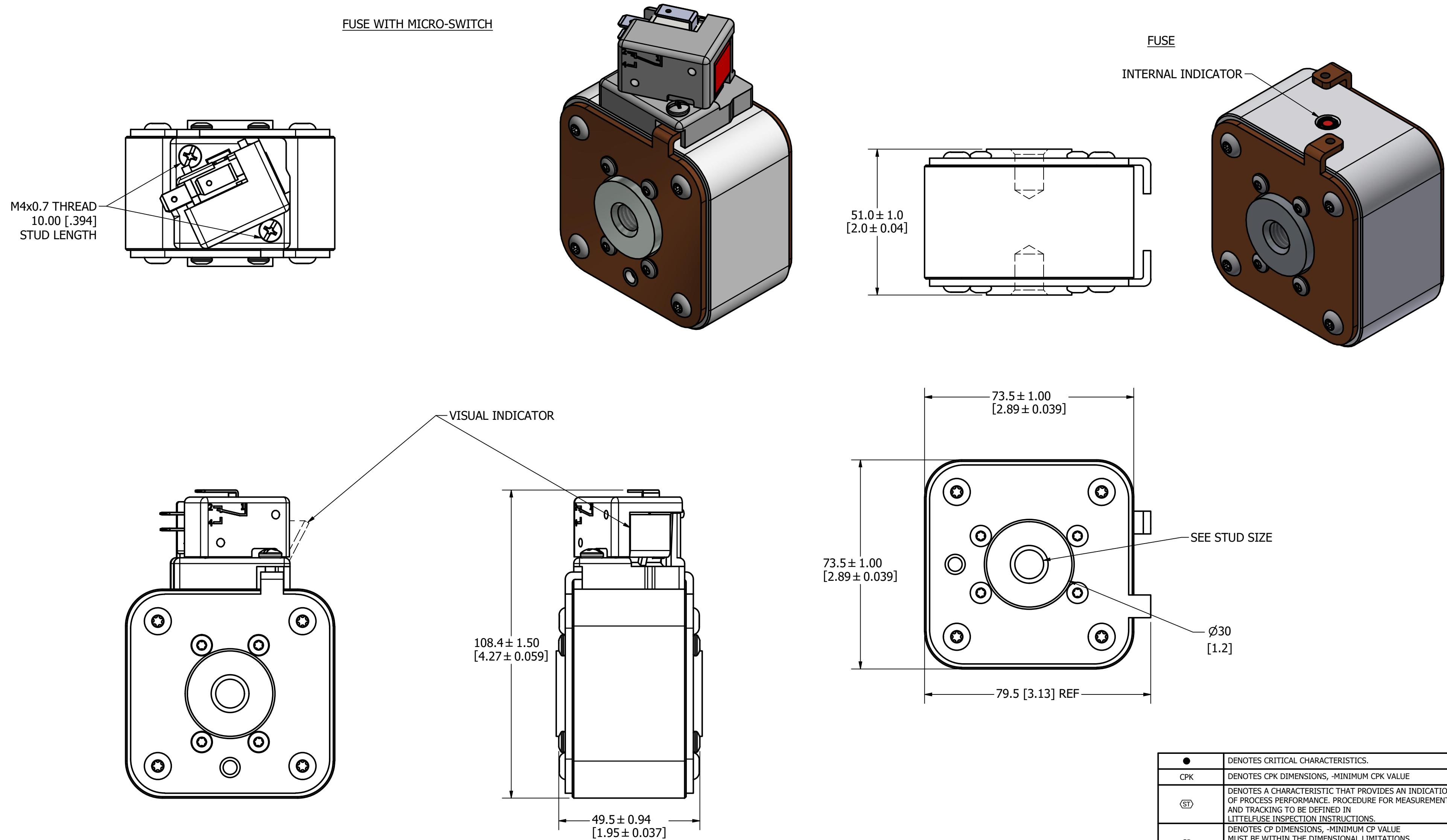
FUSE WITH MICRO-SWITCH
