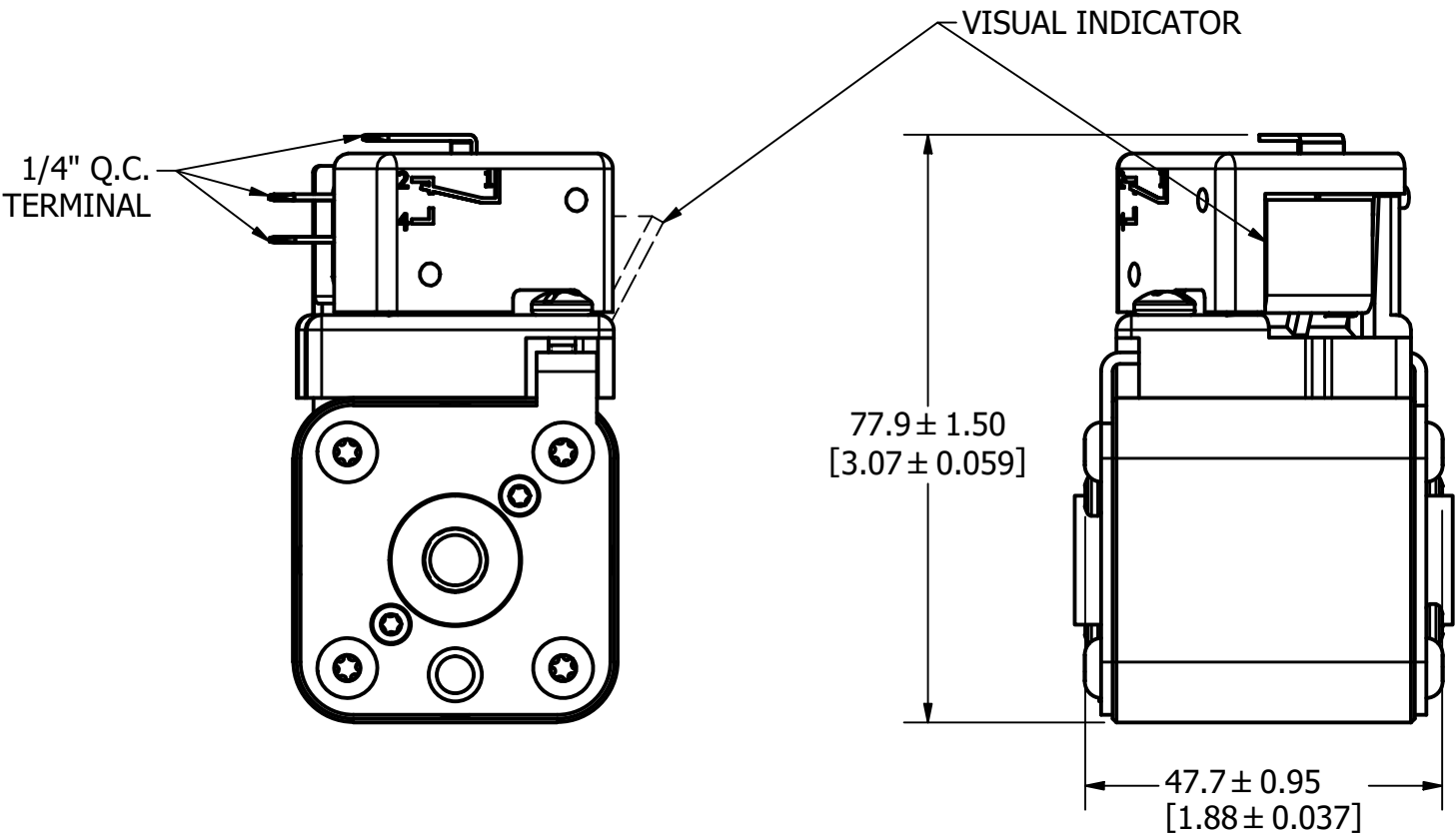
FUSE WITH MICRO-SWITCH
