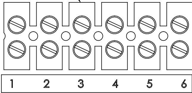
CUSTOMER CONNECTION AT CONTACTOR PANEL (ROTATED 90 DEGREES)
