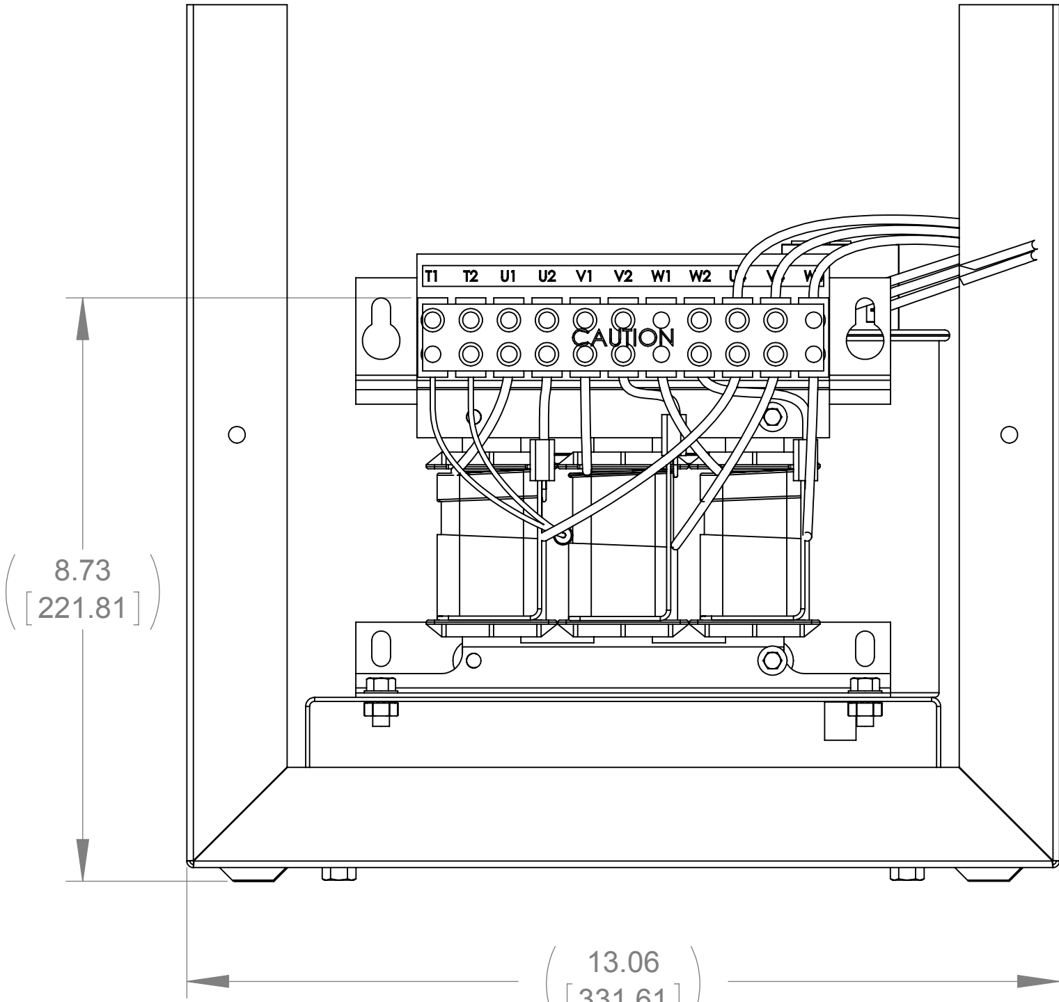
FRONT VIEW (FRONT PANEL REMOVED)
