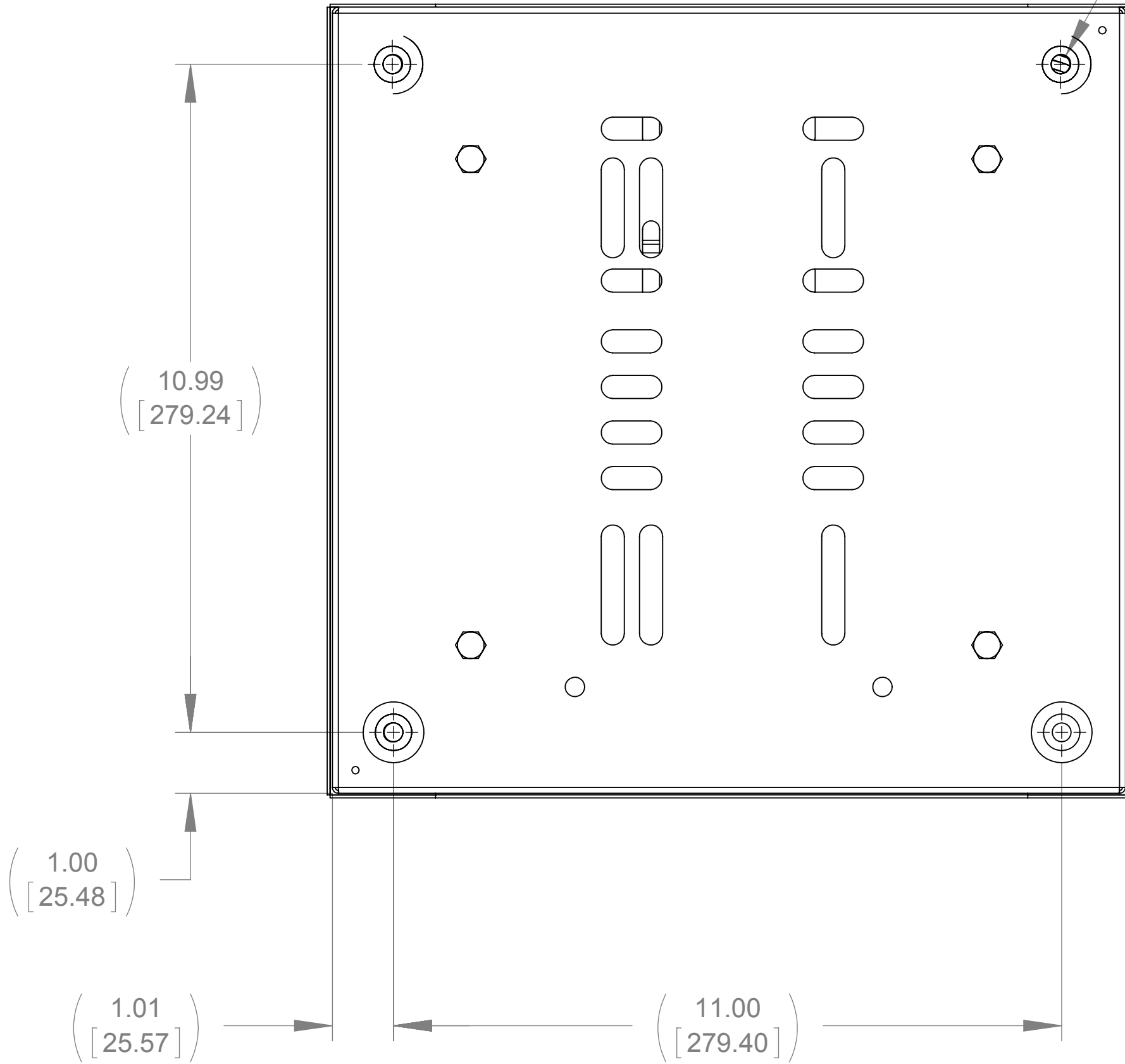
BOTTOM VIEW
