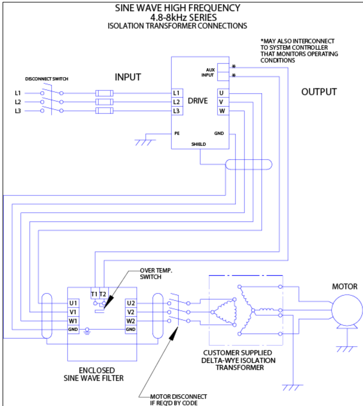
Figure 5-3: Isolation Transformer
