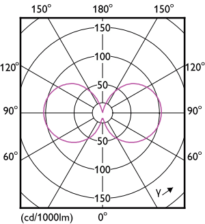
Light Distribution Diagram - 15GC/LED/840/ND E26 BB 6/1
