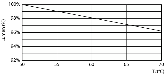
Lumen Maintenance Diagram - 14T8/MAS/48-5CCT/FF21/P/DIM 25/1
