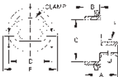
Non-watertight Connectors for Oval or Round Cable
