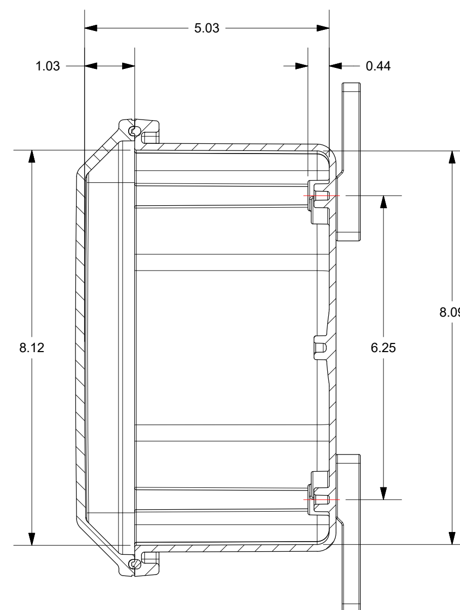
SECTION B-B
