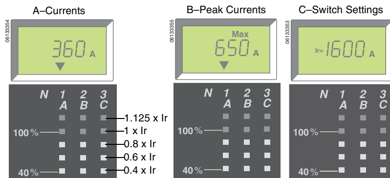
Figure 15 – Menus
