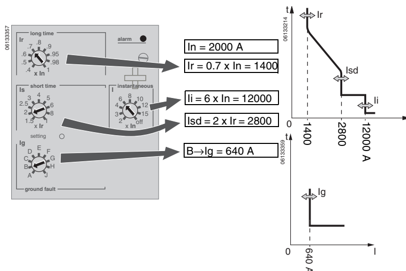
Figure 31 – Set Pickup Levels
