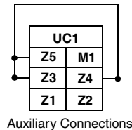
Figure 33 – Jumpered Terminals
