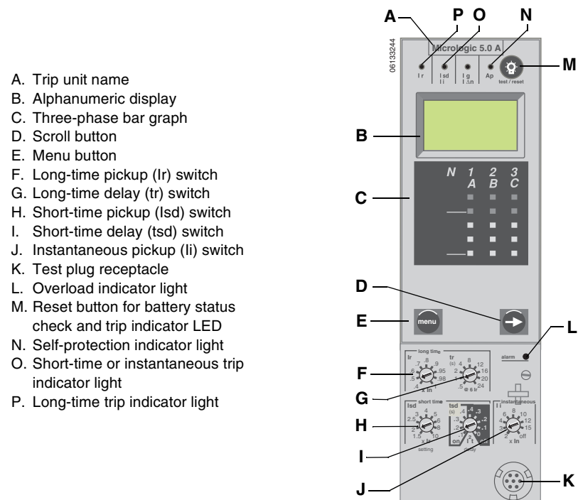
Figure 4 – 5.0A Trip Unit
