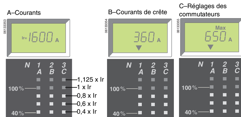
Figure 15 – Menus
