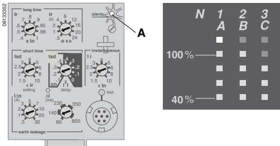
Figure 11 – Voyant de surcharge
