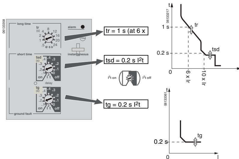
Figure 32 – Set Pickup Levels
