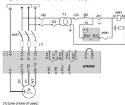
(1) Line choke (if used)
