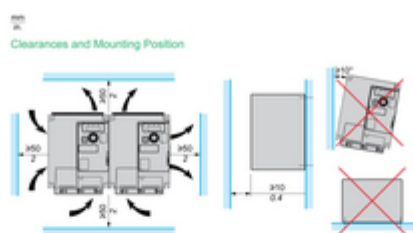
Mounting Type A
