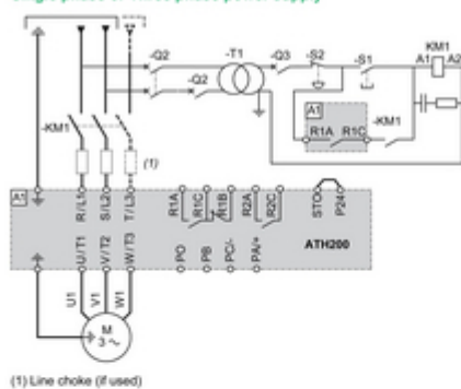
Control Block Wiring Diagram
