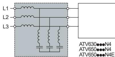
Altivar Process drive with passive filter
