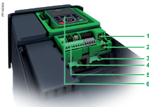
Altivar process drives ports and slots
