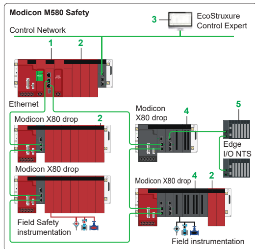
Common Safety architecture
