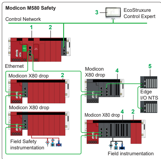
Common Safety architecture
