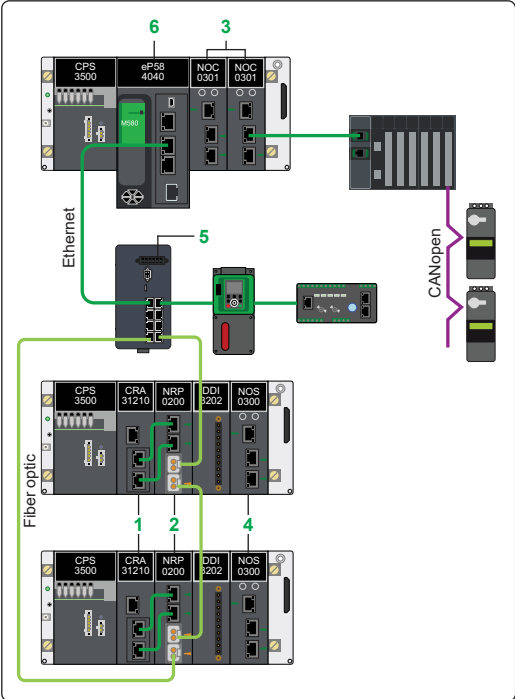
Distributed I/O architecture + remote I/O architecture (with BMENOS Modicon X80 Ethernet switch module)
