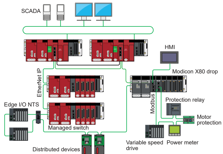
Modicon M580 Safety redundant topology
