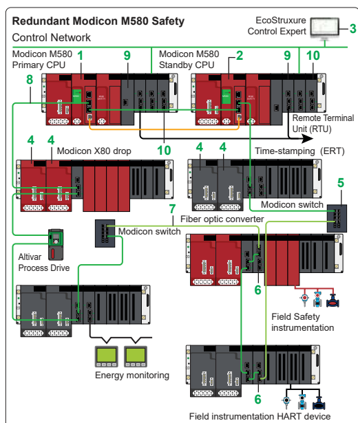
High-availability Safety architecture
