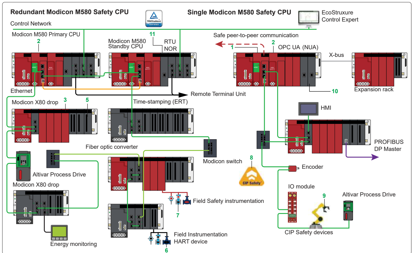
Complex Safety architecture
