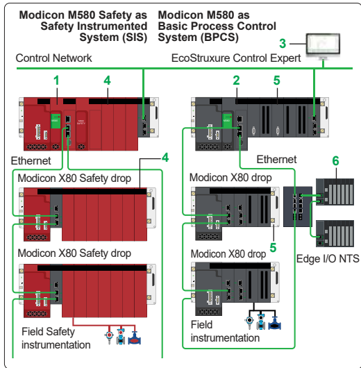
Integrated Safety architecture
