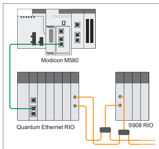
Standalone architecture example
