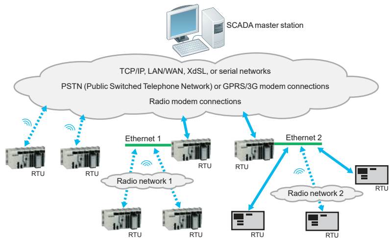
Example of an RTU system architecture
