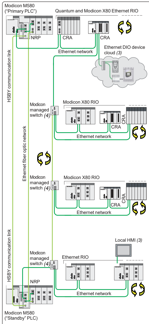
Modicon M580 Hot Standby Ethernet I/O architecture, long distance
