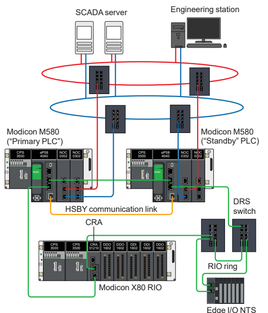
High-availability system based on mixed DIO/RIO architectures
