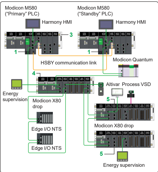
Mixed remote and distributed I/O architecture
