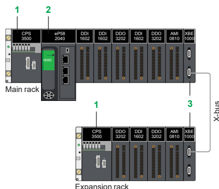
Local I/O architecture: devices on local I/O
