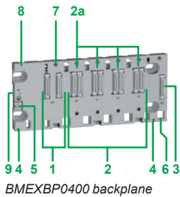
BMEXBP0400 backplane
