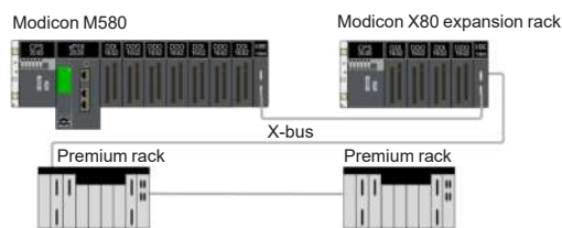
Premium X-bus extension example
