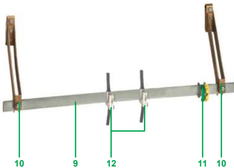
BMXXSP cable shielding connection kit
