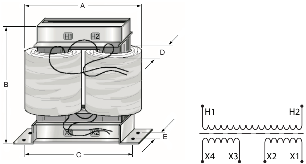
Dual Secondary—120 V and 208 V
