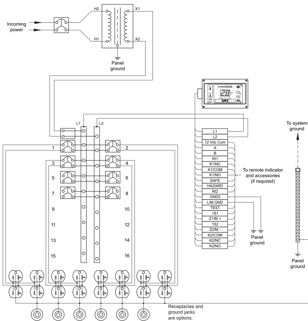
Wiring Diagram
