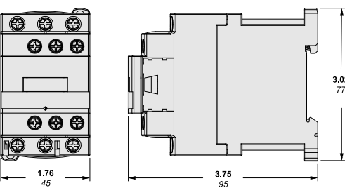
CONTACTOR WITH DC COIL
