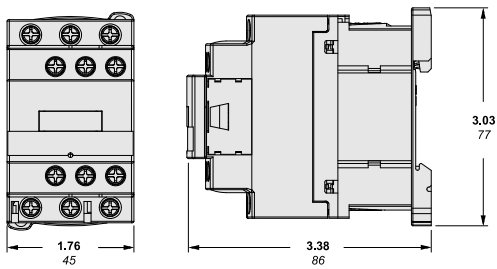
CONTACTOR WITH AC COIL
