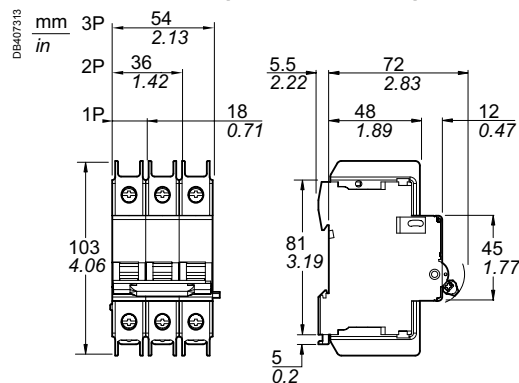
C60BPTunnel terminal
