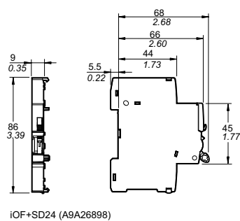
iOF+SD24 (A9A26898)
