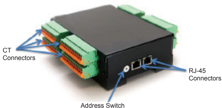
Figure 1. HDPM6000R
